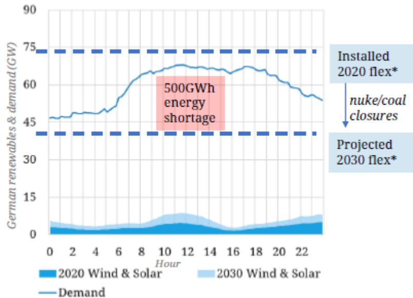
German low renewable day (GW)
